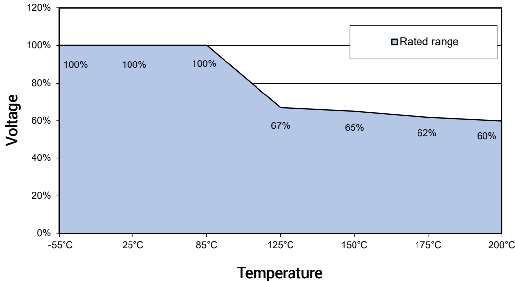
TWA-Y 200°C Voltage vs Temperature Rating
